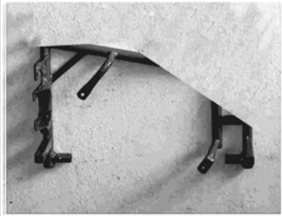
Photo from above of the frame with the section of the two supports for the exhaust system
